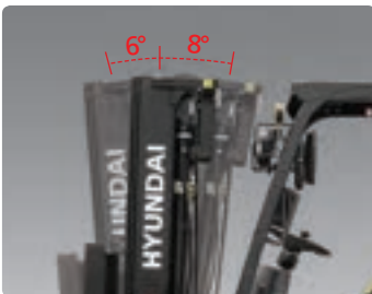
Increased Mast Tilting Angle Utilizing the mast tilting angle of 6 degrees forward and 8 degrees backward, the operator can safely and rapidly perform loading and unloading jobs.
