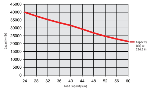
H180 (1401) Load Center Lifting Capacity Diagram
