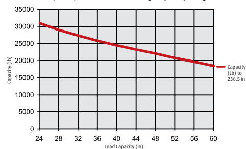
H140 (1401) Load Center Lifting Capacity Diagram
