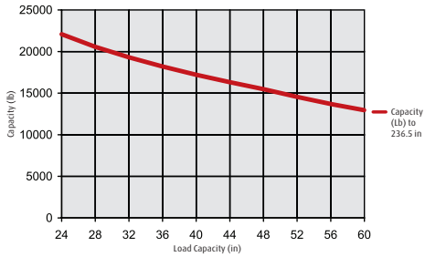
Load Center Lifting Capacity Diagram
