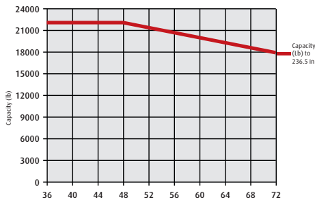
Load Center Lifting Capacity Diagram
