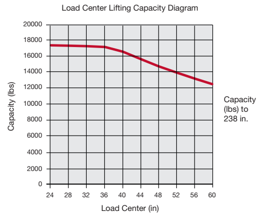
E80/900 (Simple Mast)
